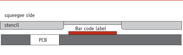
Picture 2: Cross section of Step-down on the PCB side
