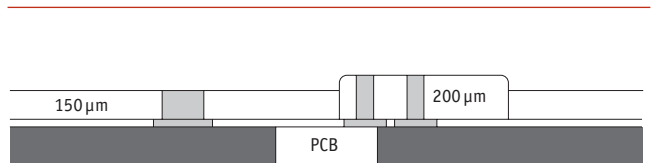
Picture 1a: Cross section of a PatchWork® stencil – step-up
